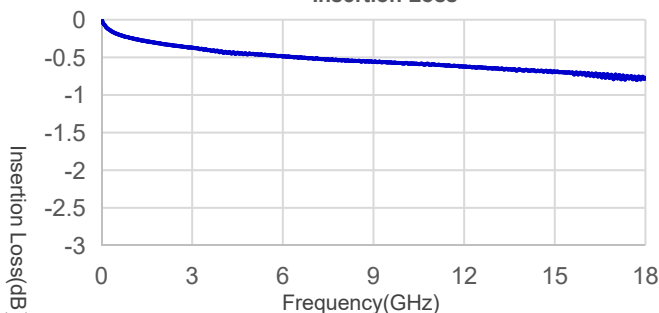
A81-SMAMSMAM-1m Insertion Loss
