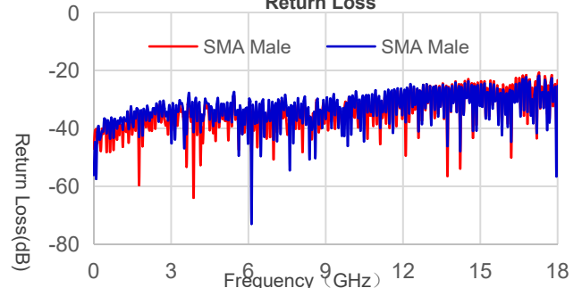
A81-SMAMSMAM-1m Return Loss
