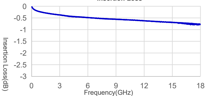
A81-SMAMNWM-1m Insertion Loss
