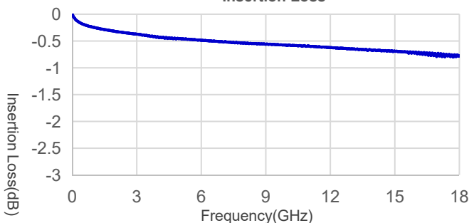
A81-NMNM-1m Insertion Loss
