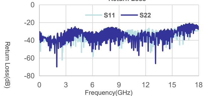
A81-NMNM-1m Return Loss
